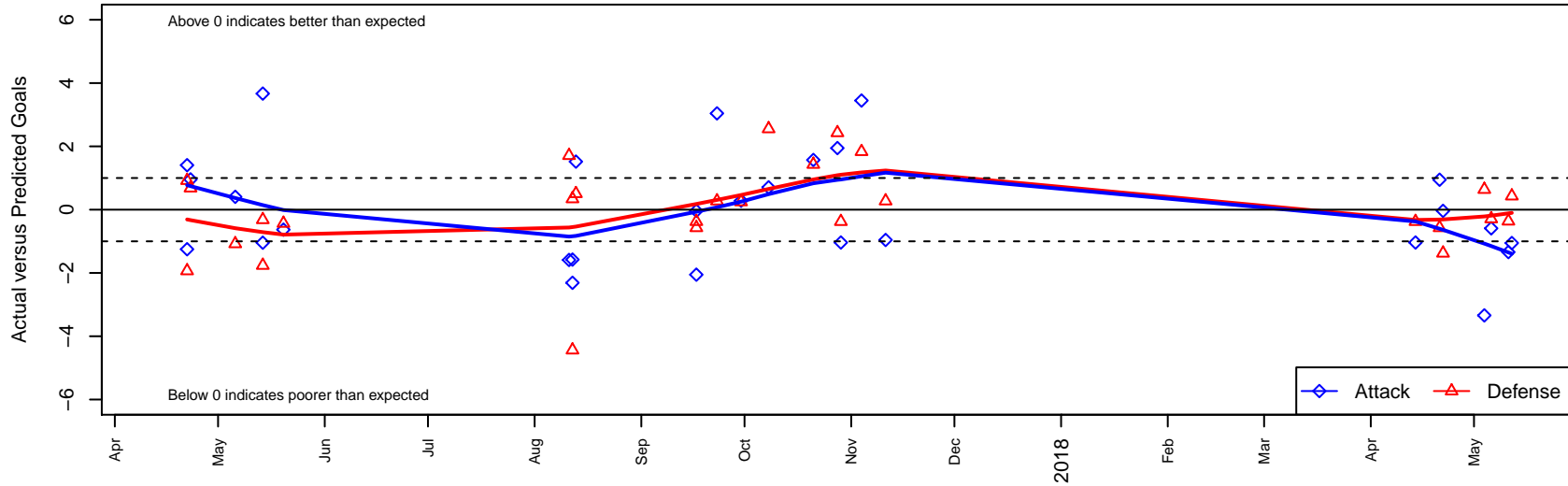
Hawks SC B04 Dots are actual minus expected GF (blue circles) and GA (red triangles). Blue line is smoothed change in attack strength. Red is smoothed change in defense strength.
